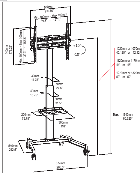
Quick-Release Spring Lock effortless adjusting height
